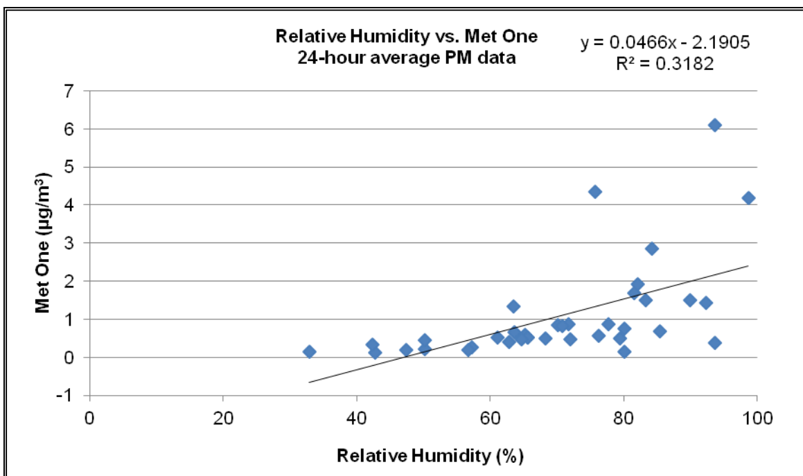
Figure 3.5.1-5. RH vs. Met One Model 831 24-hour averaged data.
