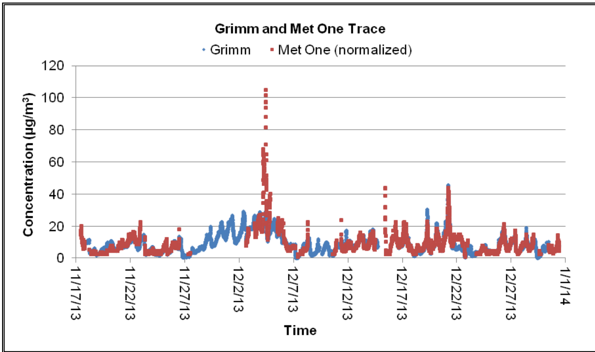
Figure 3.5.1-8. Grimm and normalized Met One Model 831 data (5-min averages) against time.
