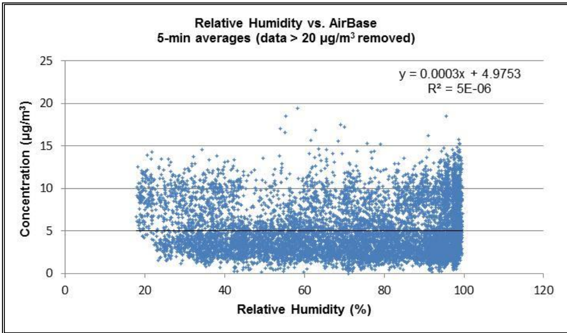
Figure 3.1.1-6. RH vs. AirBase (5-min averages) with data > 20 µg/m³ removed.
