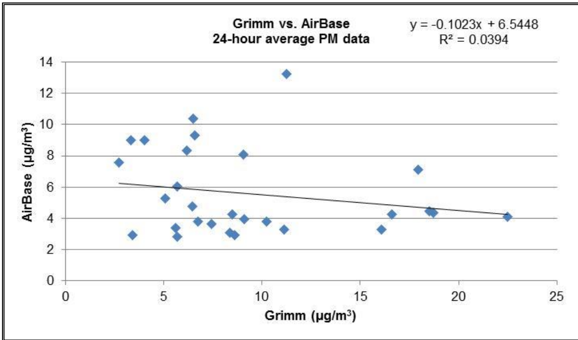
Figure 3.1.1-2. 24-hour time-averaged PM data comparing the Grimm reference sampler with the AirBase CanarIT PM sensor.
