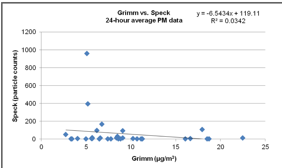
Figure 3.3.1-2. 24-hour time-averaged PM data comparing the Grimm reference sampler with the Speck.
