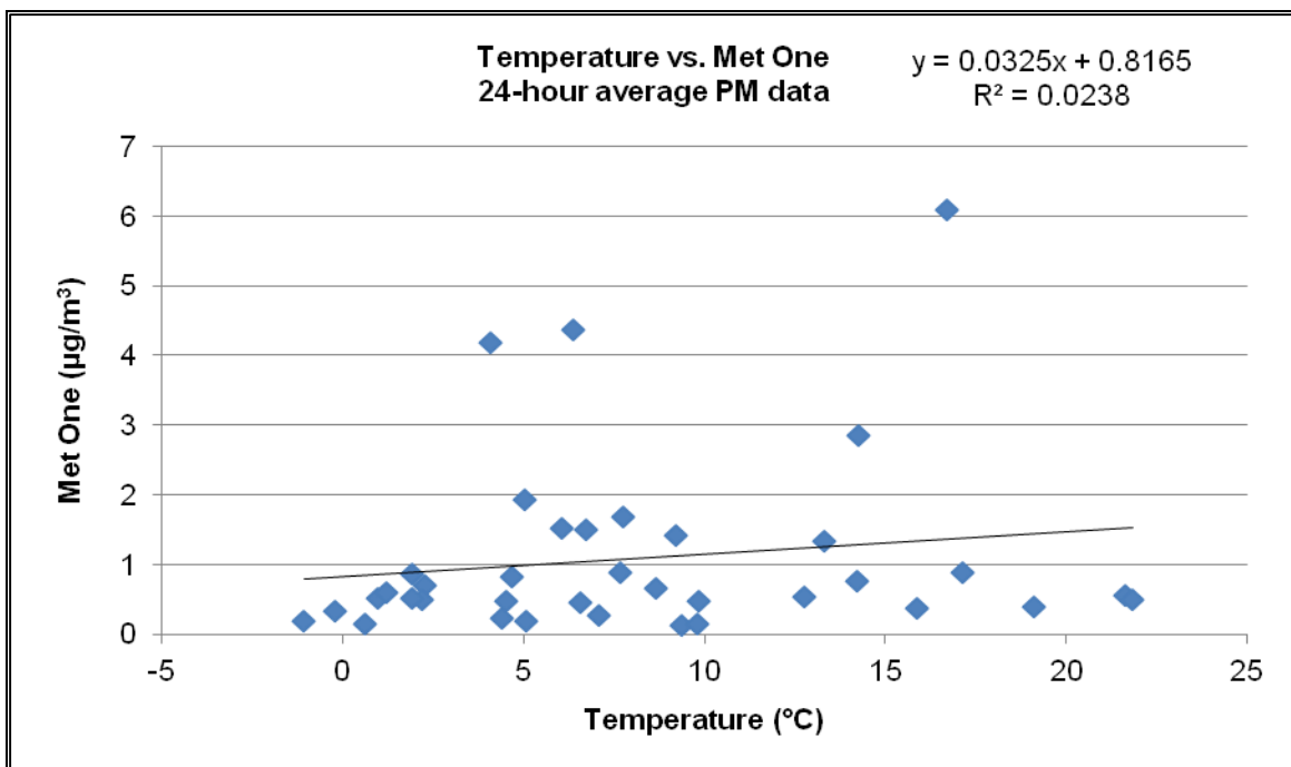
Figure 3.5.1-4. Temperature vs. Met One Model 831 24-hour averaged data.
