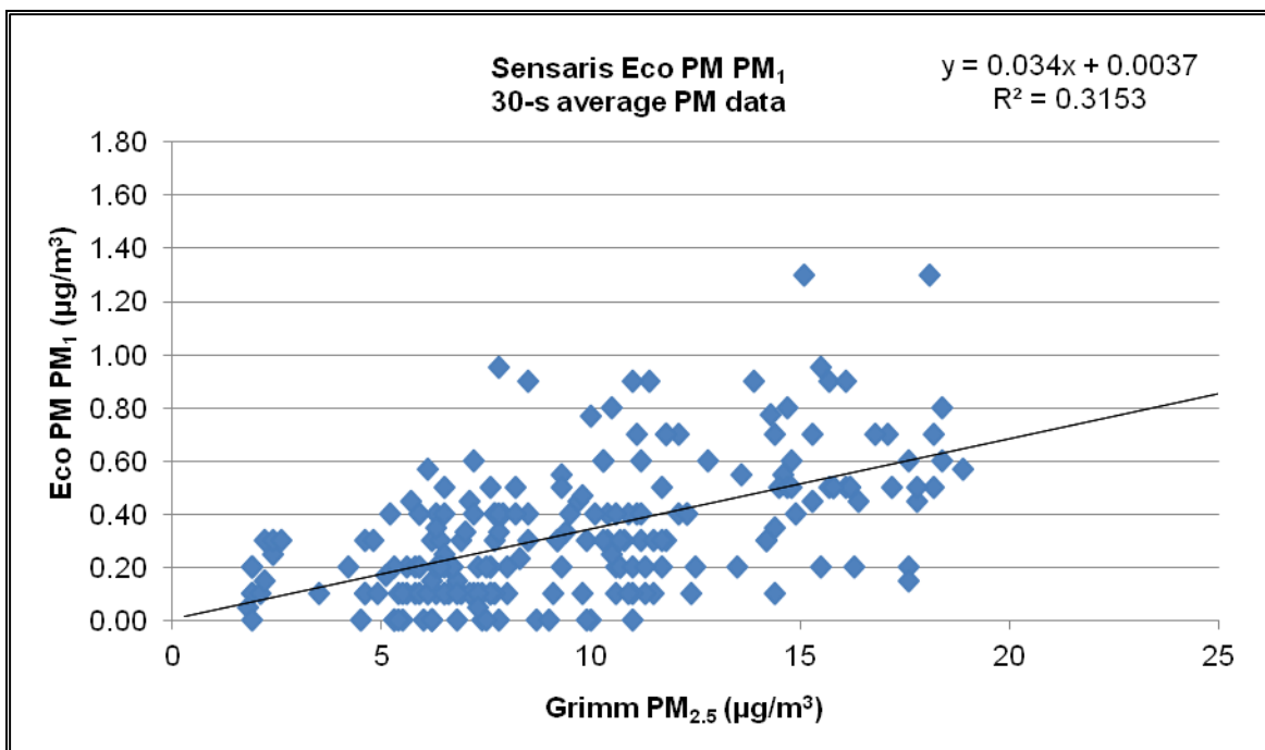
Figure 3.7.1-2. 30-s time-averaged PM data comparing the Grimm reference sampler with the Eco PM sensor.
